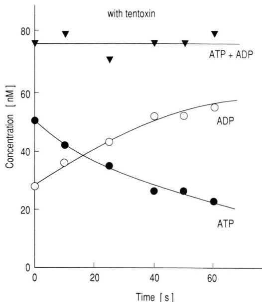
Fig. 3. Single-site ATP hydrolysis: The proteoliposomes ( [\text{CF}_0\text{F}_1] = 1\ \mu\text{M} ) were preincubated with 4\ \mu\text{M} tentoxin for 10 min. Then, the enzyme was activated by a \text{pH}/\Delta\Psi jump and ATP was added. During the reaction 4\ \mu\text{M} tentoxin was present. The concentration of free ATP and the sum of free (ATP + ADP) were measured as a function of reaction time. The concentration of free ADP was calculated from the difference between both measurements.
