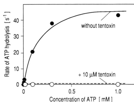
Fig. 4. Rate of ATP hydrolysis as a function of the ATP concentration. \text{CF}_0\text{F}_1 ( 1.4\ \mu\text{M} ) was preincubated either without or with 10\ \mu\text{M} tentoxin for 10 min, then the enzyme was activated by a \text{pH}/\Delta\Psi jump and the reaction was started by addition of \gamma\text{-}^{32}\text{P}\text{-ATP} and 10\ \text{mM} \text{NH}_4\text{Cl} (final concentration).
